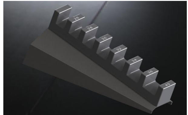
Casing 40-36-34-32-30-28-26 mm; Range 40-26 Socket Steel 1.4301 VA obliquely Artikel:101706 / Price 186,00 Euro / pcs.
